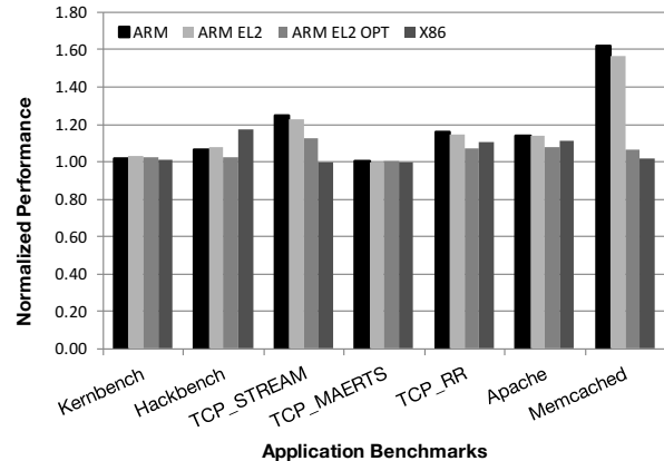
Figure 2: Application Benchmark Performance
